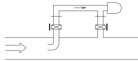
WITH PITOT TUBE (TOP VIEW) UNIT MOUNTS ON THE SIDE OF MAIN PIPE
