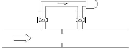
AROUND ORIFICE PLATE OR VALVE
